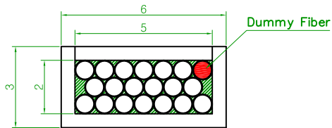
View A (19 Fibers) Array Bundle End Scale x10
