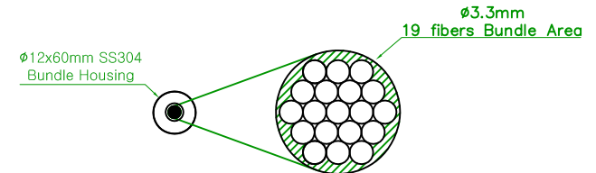
View B (19 Fibers) UV Light Input Scale: x10
